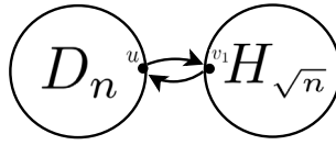
Fig. 5. The construction in Example 3.
