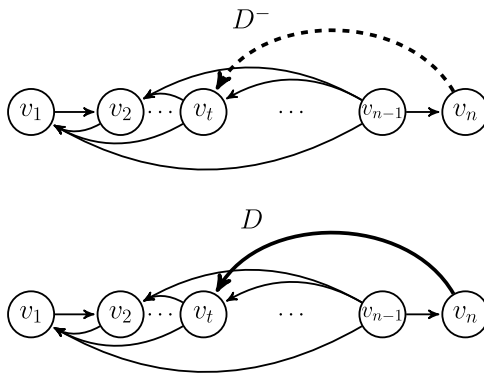
Fig. 3. D and D^- . A dashed edge indicates the absence of that edge.
