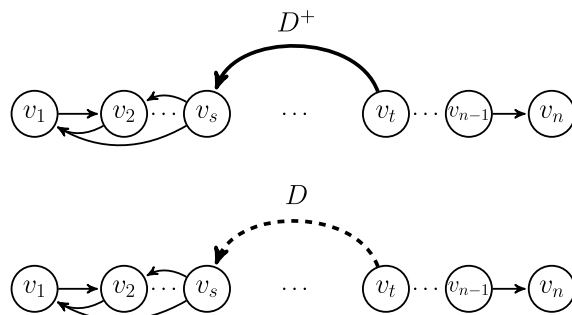
Fig. 2. D and D^+ . A dashed edge indicates the absence of that edge.
