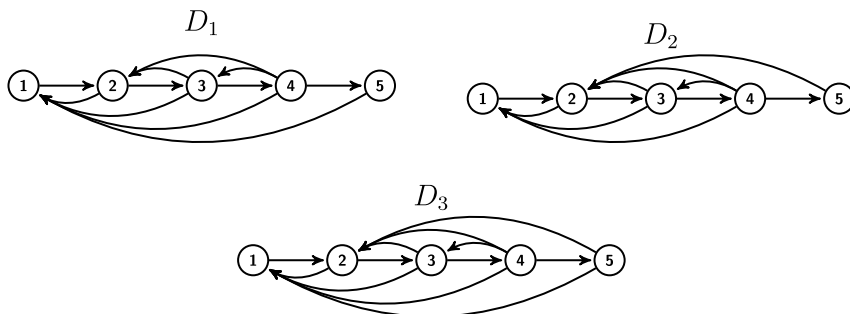
Fig. 1. The three constructions D_1 , D_2 , D_3 for n = 5 .
