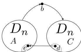
Fig. 4. The construction in Example 2.
